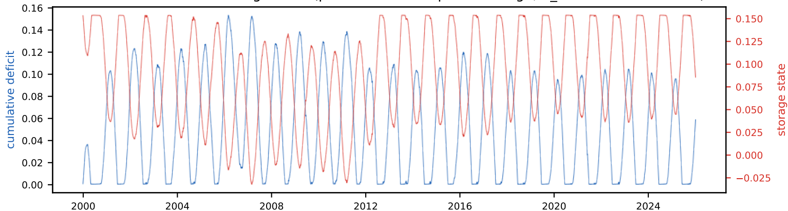
Cumulative deficit & storage state (peak deficit = required storage, S_{\text{tot}} =15.4% of annual)
