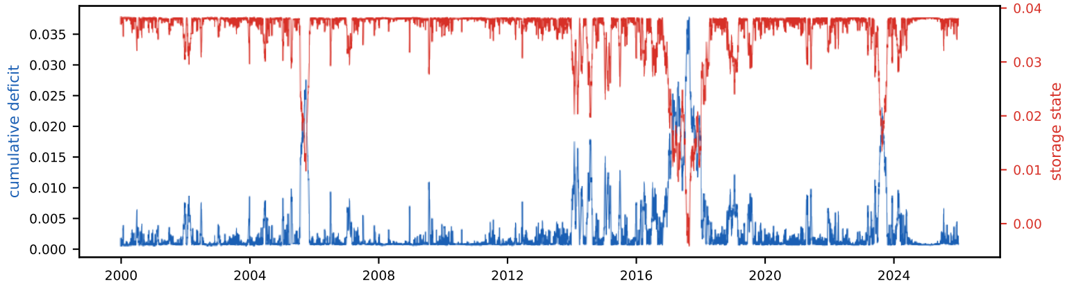
Cumulative deficit & storage state (peak deficit = required storage, S_{\text{tot}} =3.9% of annual)
