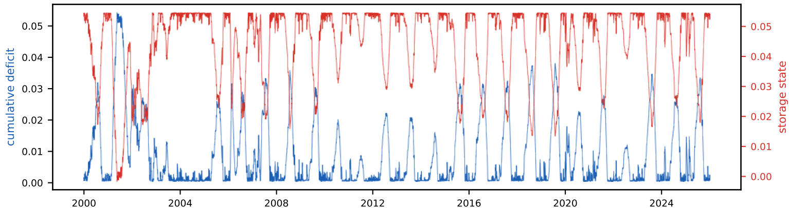
Cumulative deficit & storage state (peak deficit = required storage, S_{\text{tot}} =5.5% of annual)
