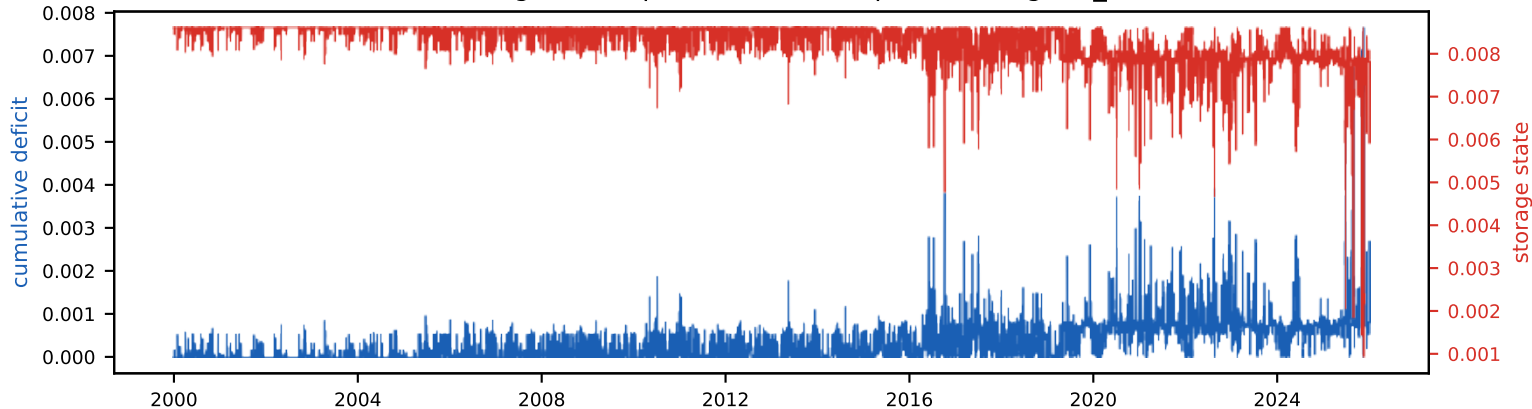
Cumulative deficit & storage state (peak deficit = required storage, S_{\text{tot}}=0.9\% of annual)
