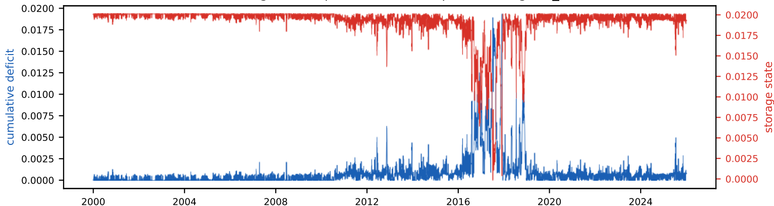
Cumulative deficit & storage state (peak deficit = required storage, S_{tot} =2.0% of annual)
