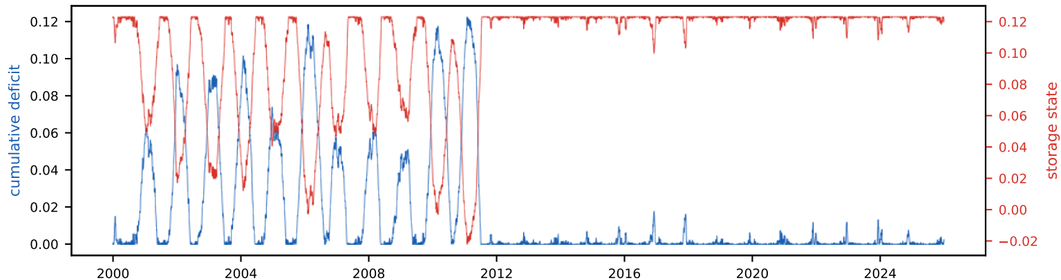
Cumulative deficit & storage state (peak deficit = required storage, S_{\text{tot}} =12.3% of annual)
