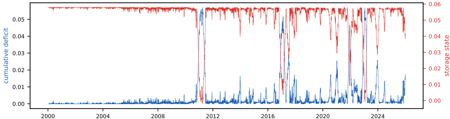
Cumulative deficit & storage state (peak deficit = required storage, S_{\text{tot}} =5.8% of annual)
