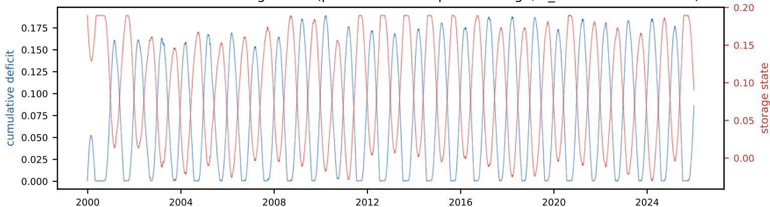
Cumulative deficit & storage state (peak deficit = required storage, S_{\text{tot}} =19.0% of annual)
