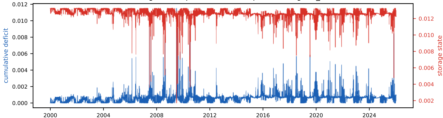
Cumulative deficit & storage state (peak deficit = required storage, S_{\text{tot}}=1.3\% of annual)
