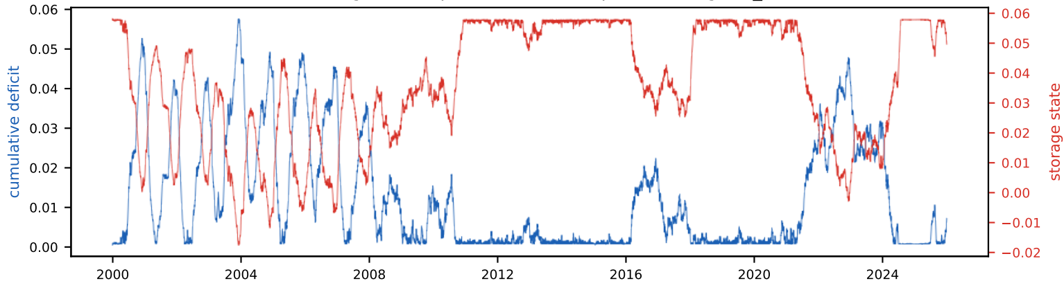
Cumulative deficit & storage state (peak deficit = required storage, S_{\text{tot}} =5.9% of annual)
