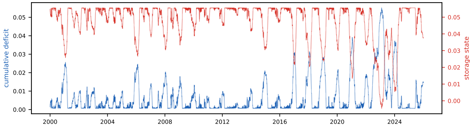
Cumulative deficit & storage state (peak deficit = required storage, S_{\text{tot}} =5.6% of annual)
