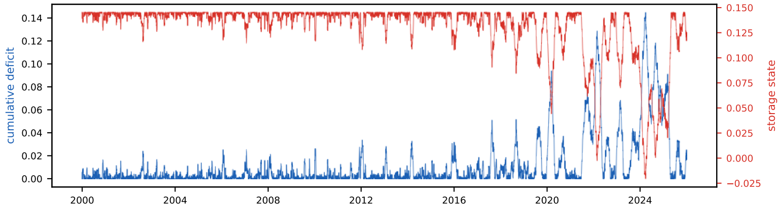
Cumulative deficit & storage state (peak deficit = required storage, S_{\text{tot}} =14.5% of annual)
