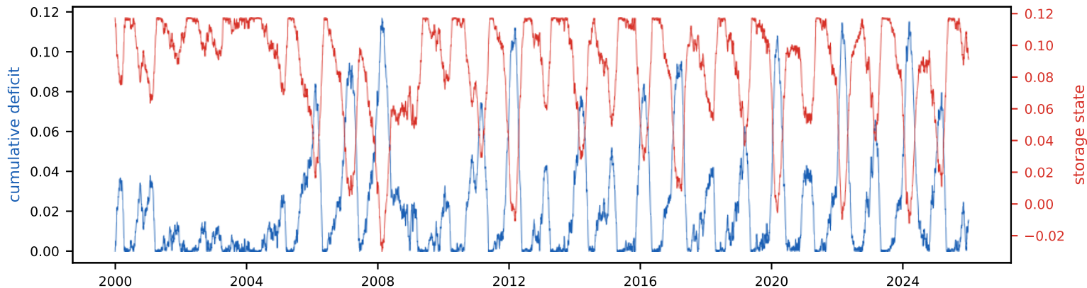
Cumulative deficit & storage state (peak deficit = required storage, S_{\text{tot}} =11.7% of annual)
