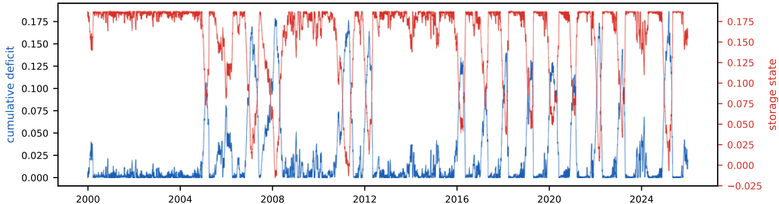
Cumulative deficit & storage state (peak deficit = required storage, S_{\text{tot}} =18.7% of annual)
