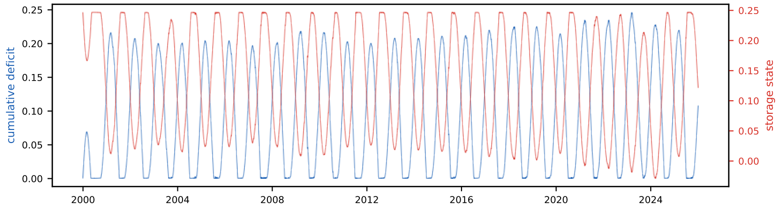
Cumulative deficit & storage state (peak deficit = required storage, S_{\text{tot}} =24.7% of annual)
