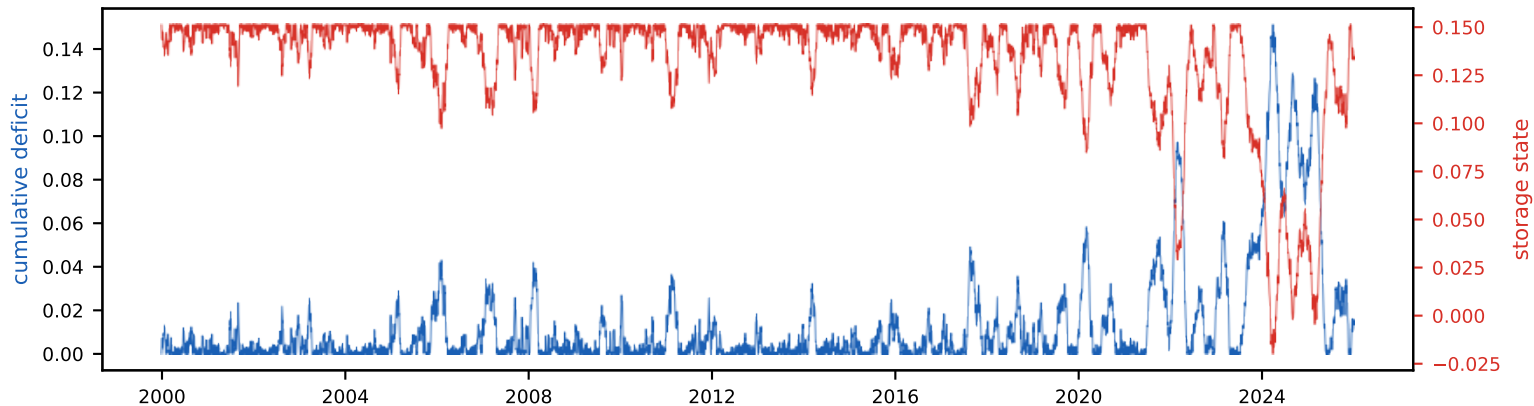
Cumulative deficit & storage state (peak deficit = required storage, S_{\text{tot}} =15.1% of annual)
