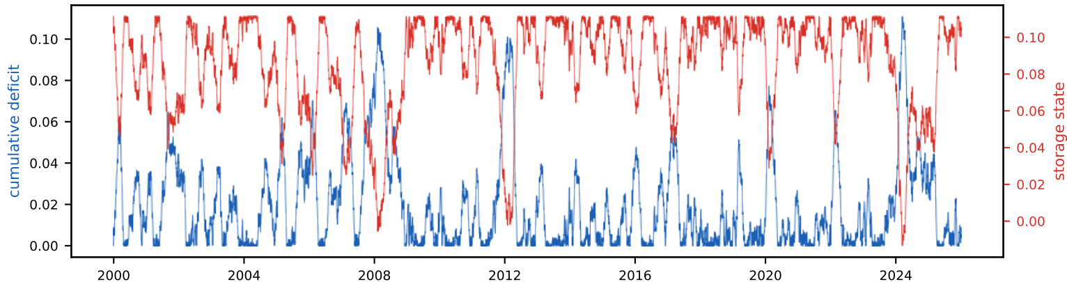
Cumulative deficit & storage state (peak deficit = required storage, S_{\text{tot}} =11.1% of annual)
