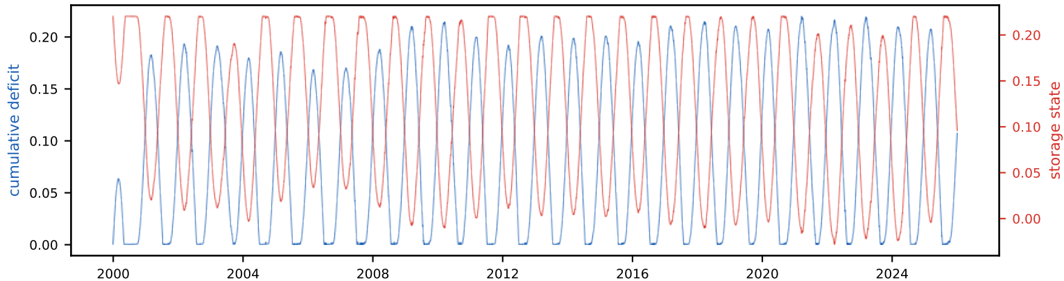
Cumulative deficit & storage state (peak deficit = required storage, S_{\text{tot}} =22.1% of annual)
