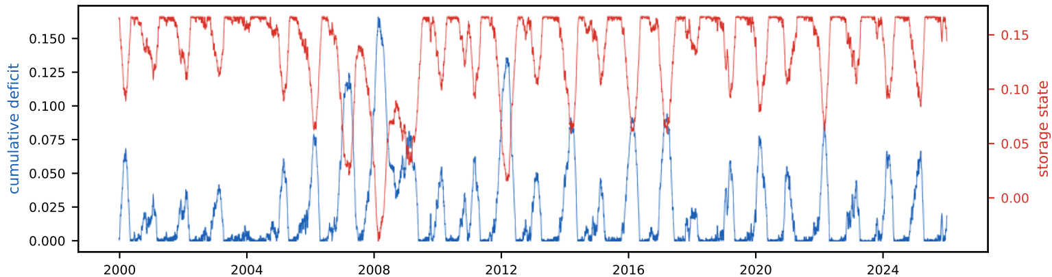
Cumulative deficit & storage state (peak deficit = required storage, S_{\text{tot}} =16.6% of annual)
