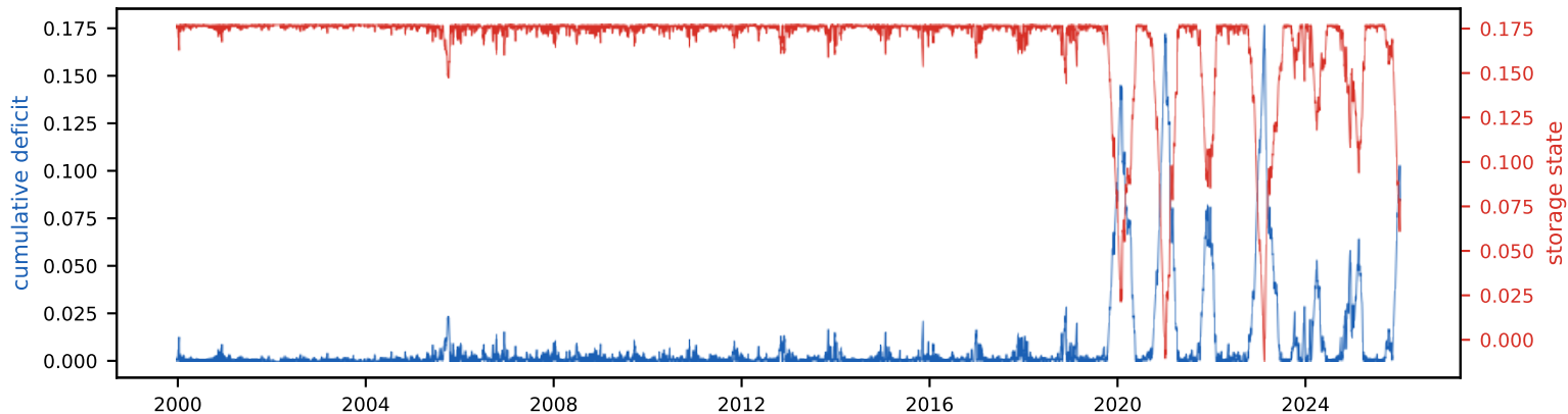
Cumulative deficit & storage state (peak deficit = required storage, S_{\text{tot}} =17.7% of annual)
