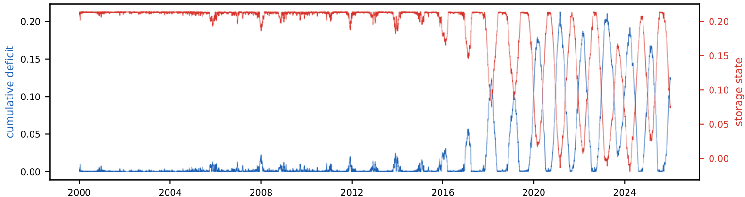
Cumulative deficit & storage state (peak deficit = required storage, S_{\text{tot}} =21.4% of annual)
