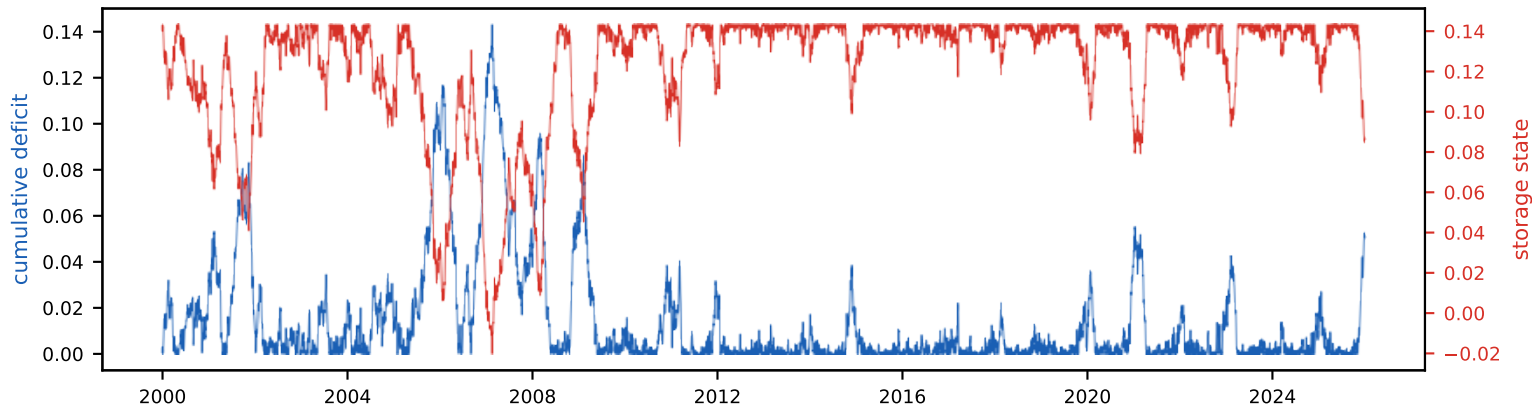
Cumulative deficit & storage state (peak deficit = required storage, S_{\text{tot}} =14.3% of annual)
