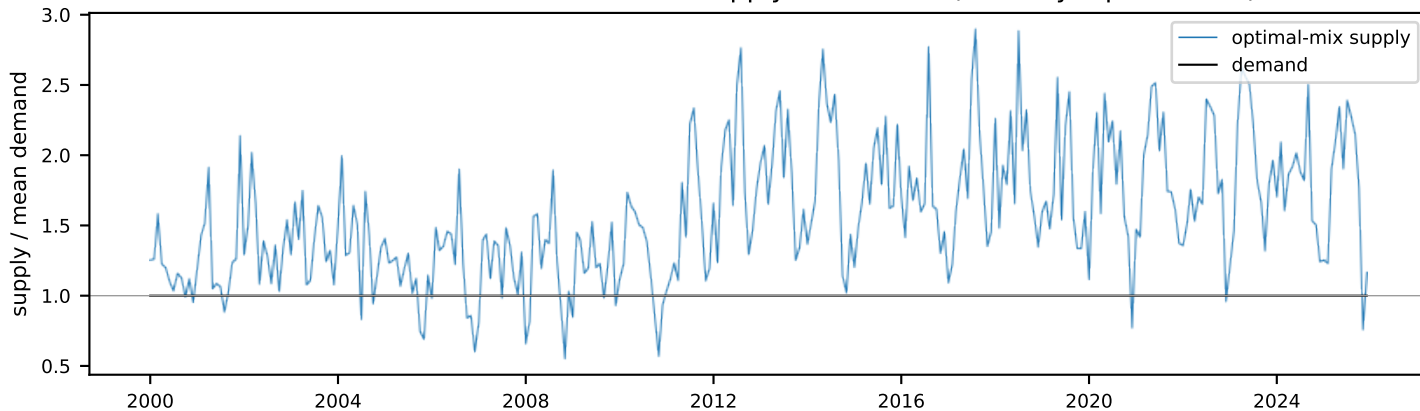
South Kazakhstan — normalized supply vs demand (monthly, optimal mix)
