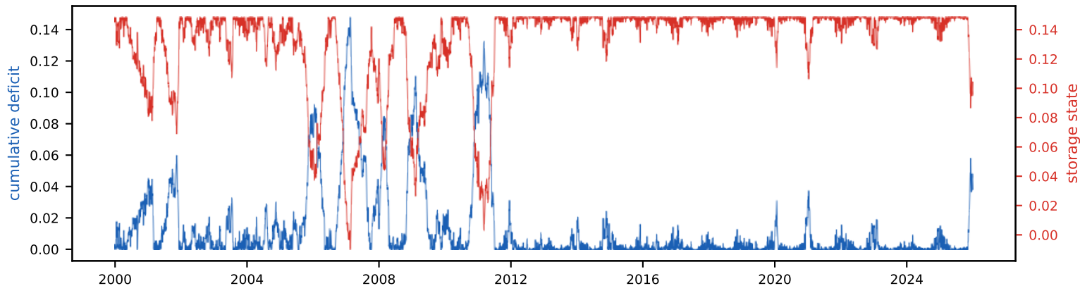
Cumulative deficit & storage state (peak deficit = required storage, S_{tot}=14.8\% of annual)
