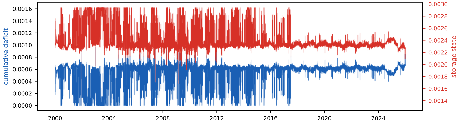
Cumulative deficit & storage state (peak deficit = required storage, S_{\text{tot}}=0.3\% of annual)
