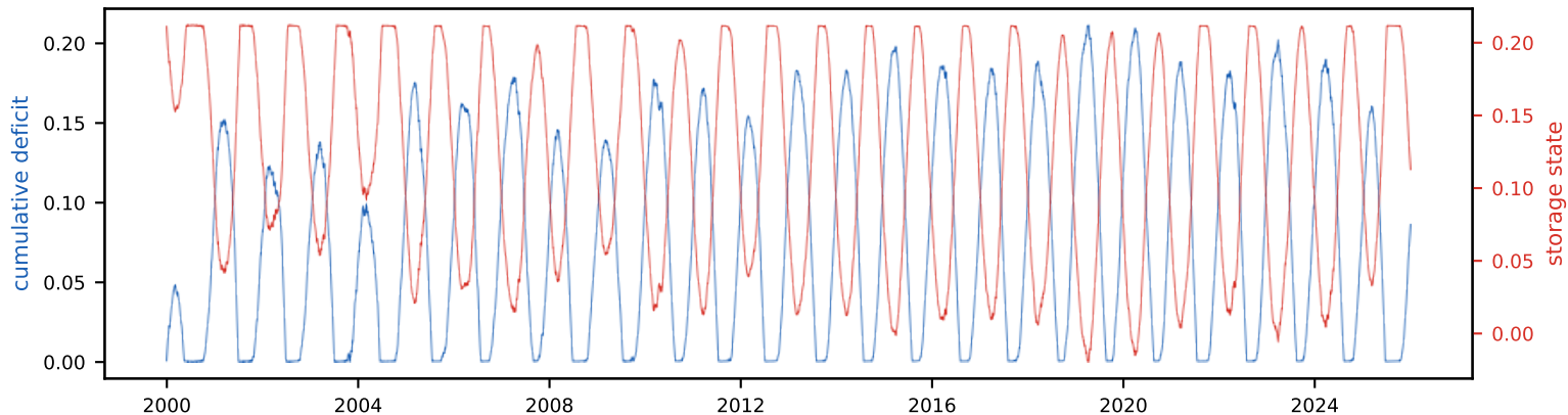
Cumulative deficit & storage state (peak deficit = required storage, S_{\text{tot}} =21.2% of annual)
