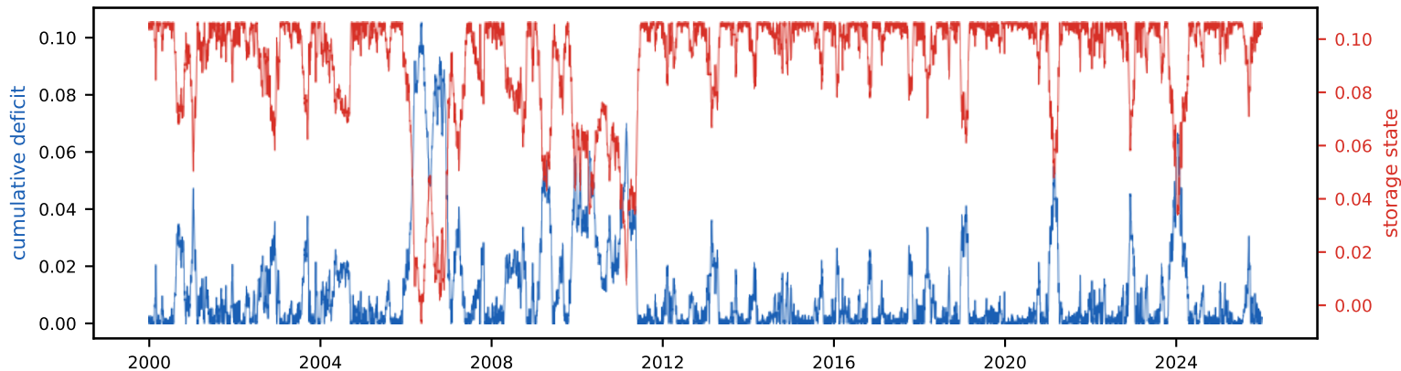
Cumulative deficit & storage state (peak deficit = required storage, S_{\text{tot}} =10.6% of annual)
