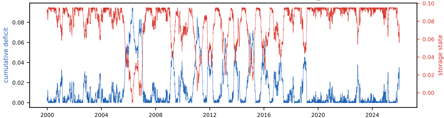
Cumulative deficit & storage state (peak deficit = required storage, S_{\text{tot}} =9.5% of annual)
