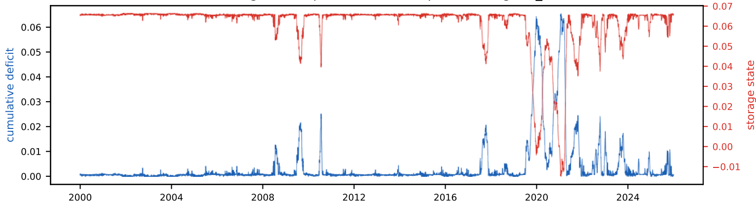
Cumulative deficit & storage state (peak deficit = required storage, S_{\text{tot}} =6.6% of annual)
