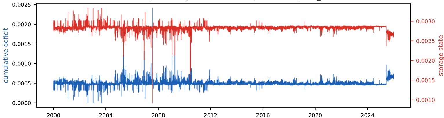
Cumulative deficit & storage state (peak deficit = required storage, S_{\text{tot}}=0.3\% of annual)
