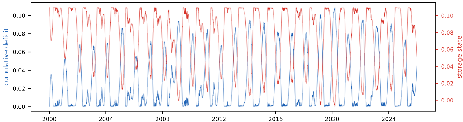
Cumulative deficit & storage state (peak deficit = required storage, S_{\text{tot}} =11.0% of annual)
