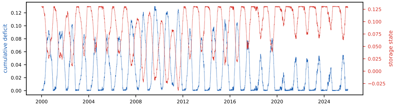
Cumulative deficit & storage state (peak deficit = required storage, S_{\text{tot}} =13.1% of annual)
