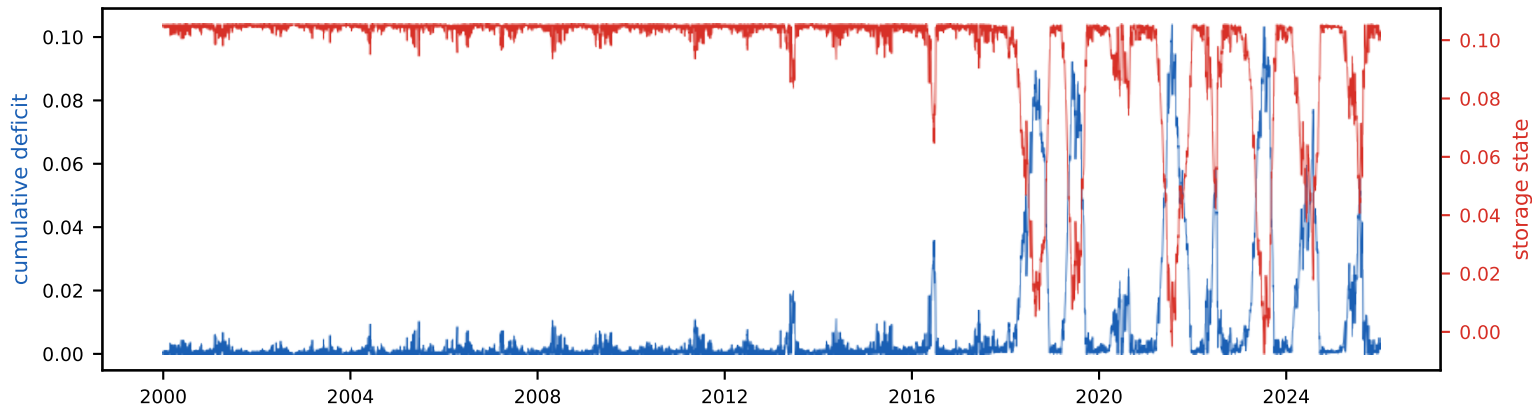
Cumulative deficit & storage state (peak deficit = required storage, S_{tot} =10.5% of annual)
