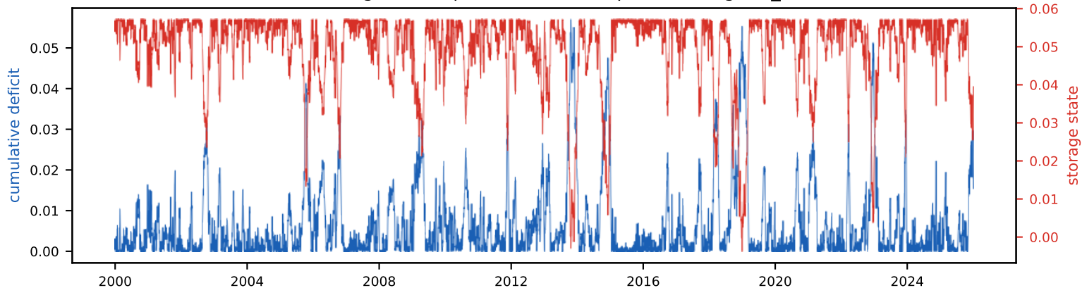
Cumulative deficit & storage state (peak deficit = required storage, S_{\text{tot}} =5.7% of annual)
