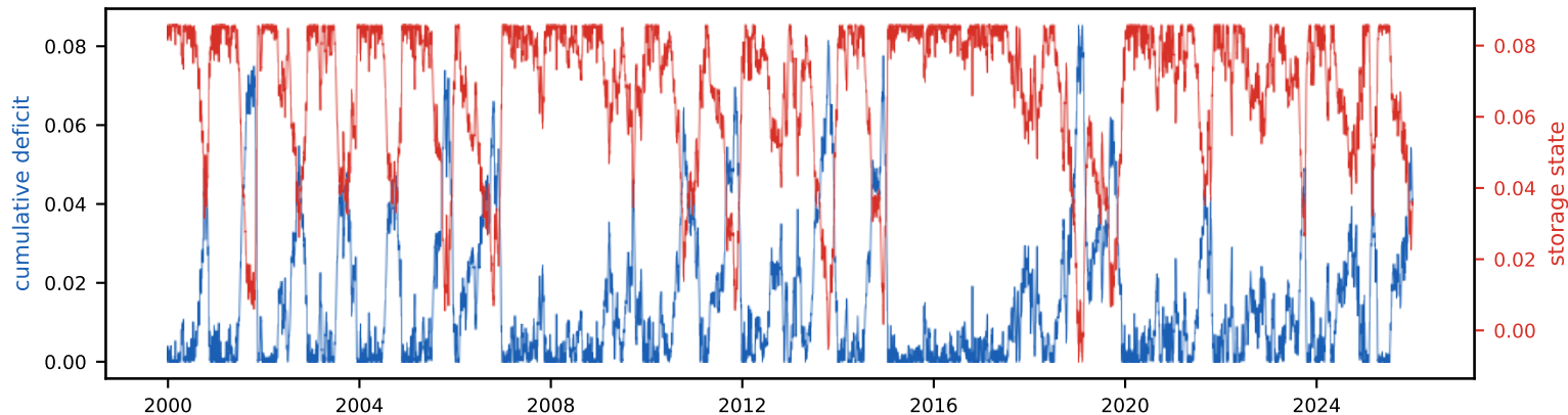
Cumulative deficit & storage state (peak deficit = required storage, S_{\text{tot}} =8.6% of annual)
