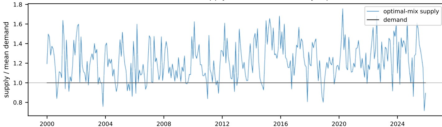
Voronezh — normalized supply vs demand (monthly, optimal mix)
