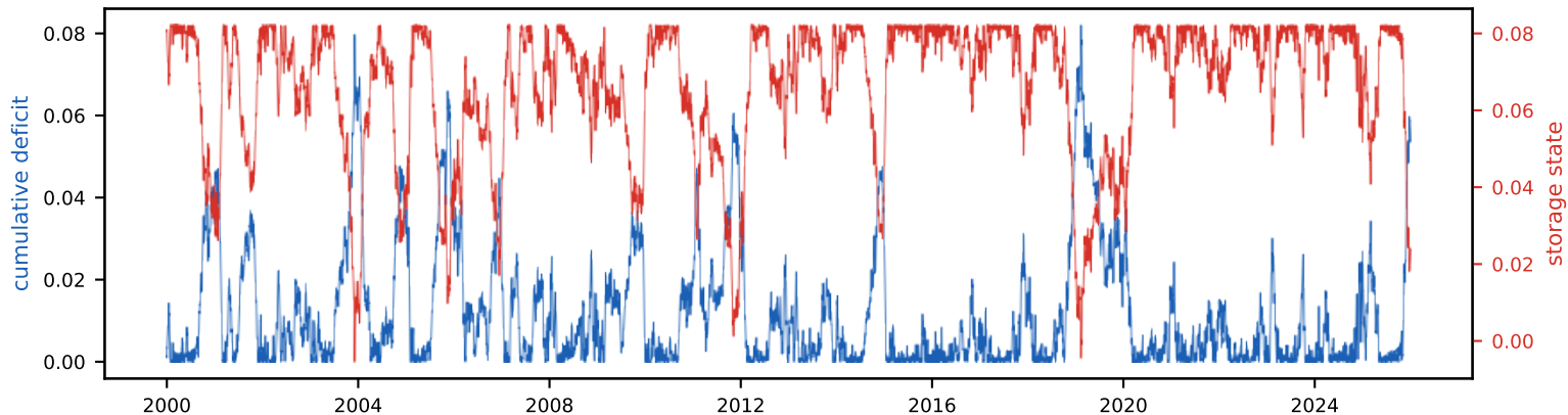
Cumulative deficit & storage state (peak deficit = required storage, S_{\text{tot}} =8.2% of annual)
