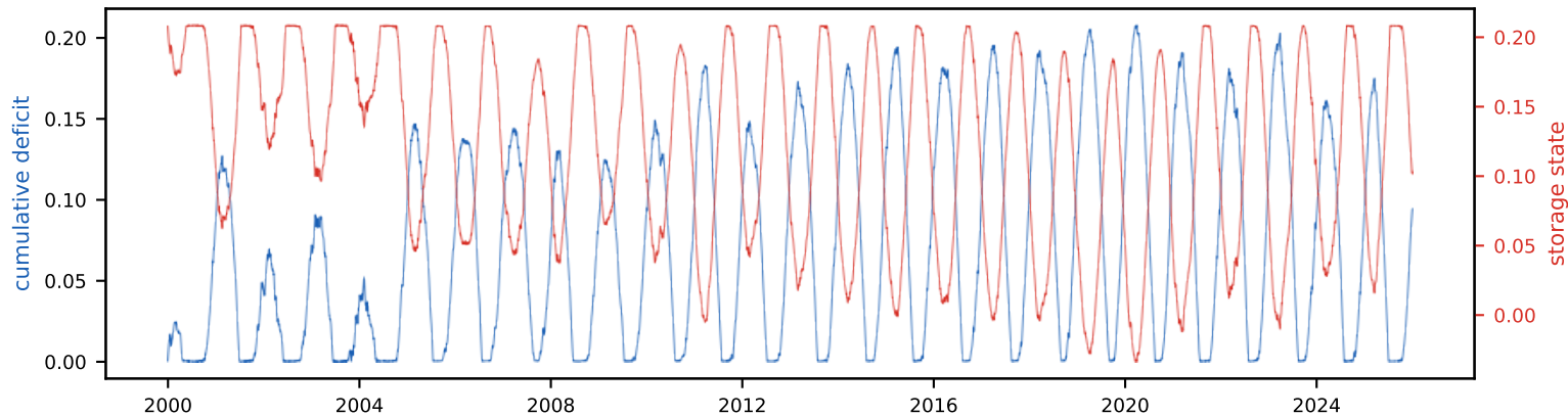
Cumulative deficit & storage state (peak deficit = required storage, S_{\text{tot}} =20.8% of annual)
