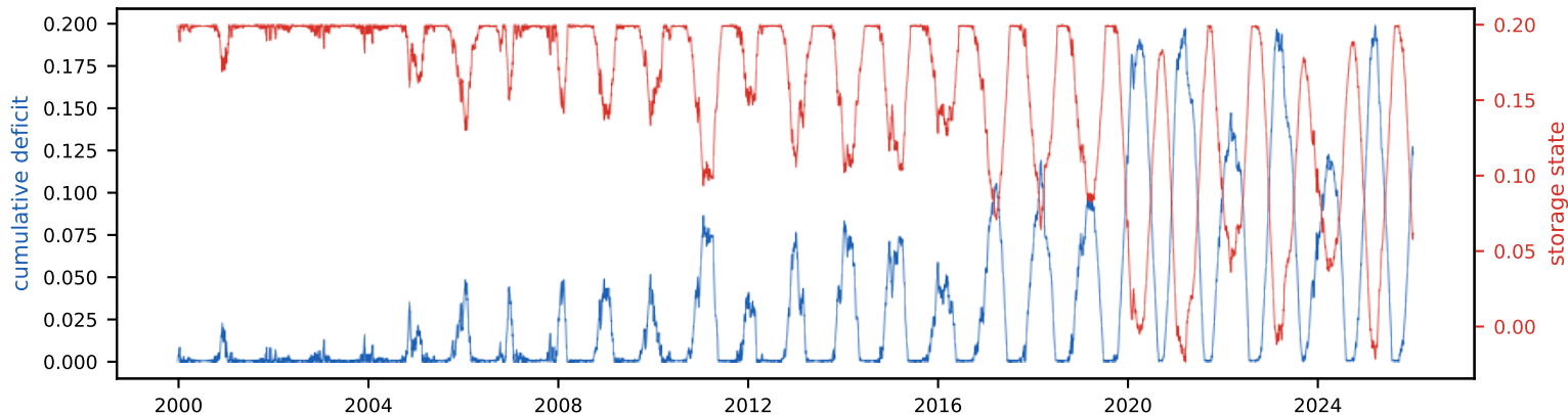
Cumulative deficit & storage state (peak deficit = required storage, S_{\text{tot}} =19.9% of annual)
