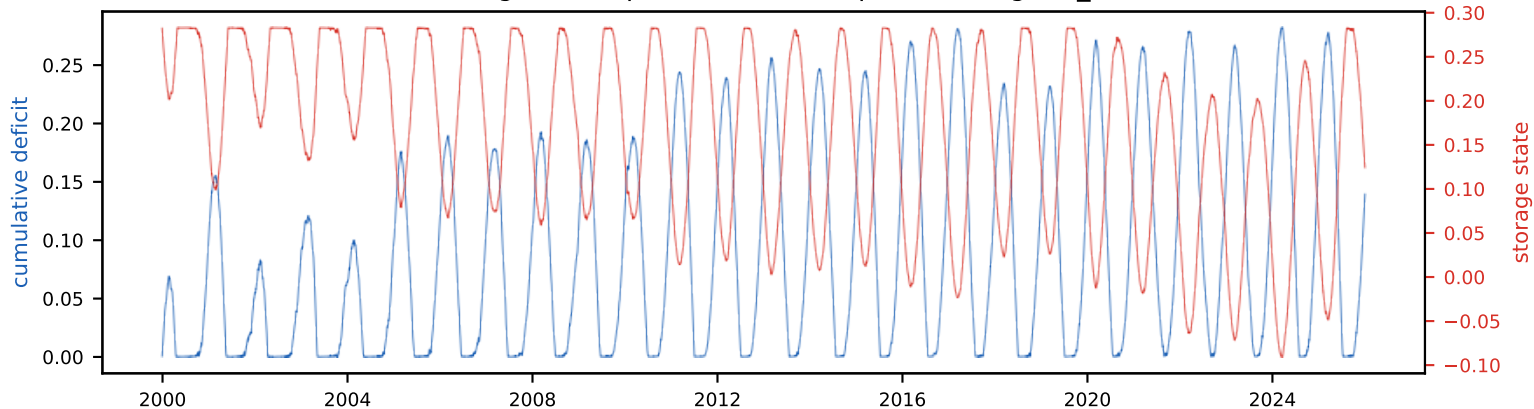
Cumulative deficit & storage state (peak deficit = required storage, S_{\text{tot}} =28.3% of annual)
