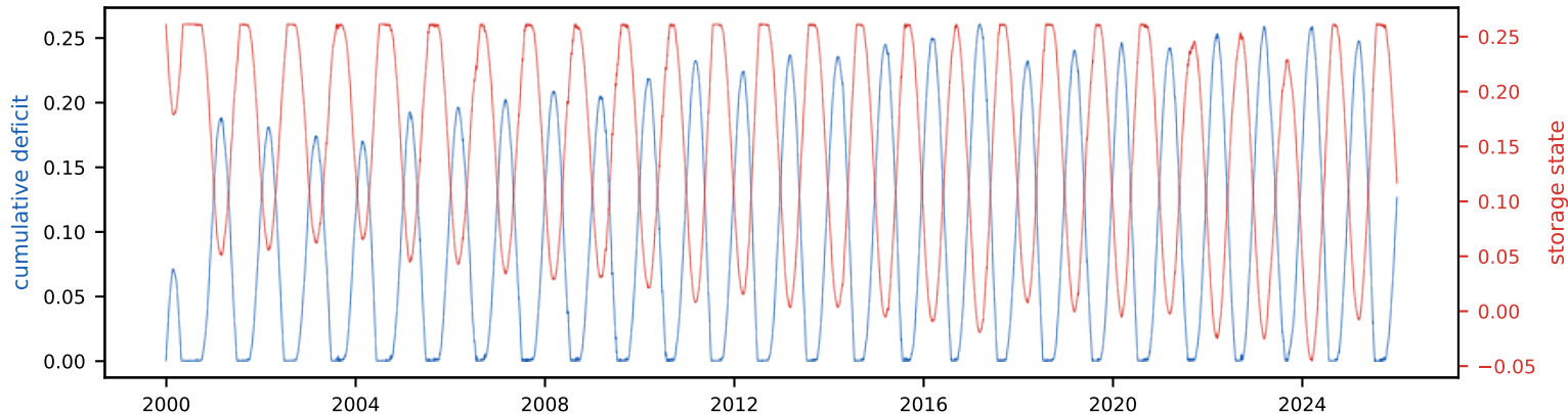
Cumulative deficit & storage state (peak deficit = required storage, S_{\text{tot}} =26.1% of annual)
