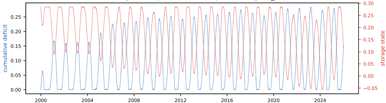
Cumulative deficit & storage state (peak deficit = required storage, S_{\text{tot}} =28.5% of annual)
