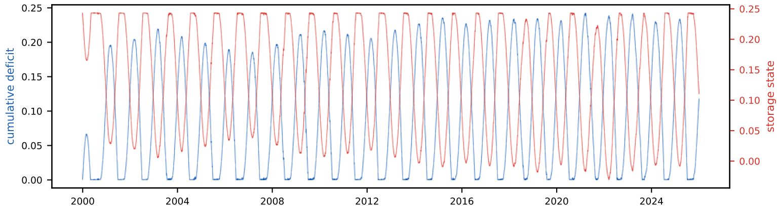
Cumulative deficit & storage state (peak deficit = required storage, S_{\text{tot}} =24.3% of annual)
