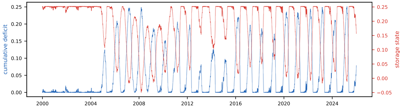
Cumulative deficit & storage state (peak deficit = required storage, S_{\text{tot}} =25.2% of annual)
