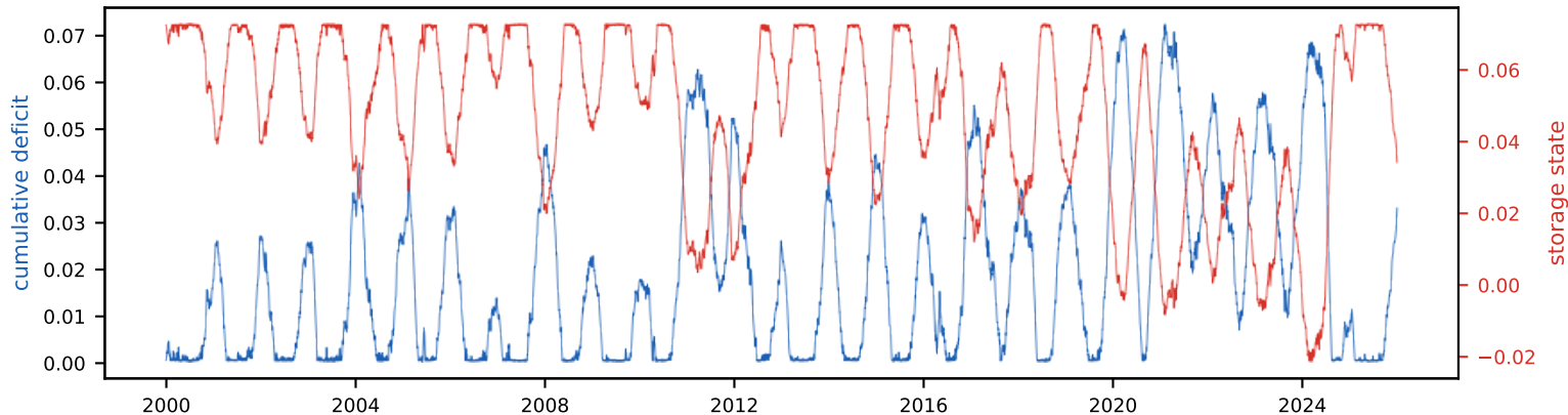
Cumulative deficit & storage state (peak deficit = required storage, S_{\text{tot}} =7.3% of annual)
