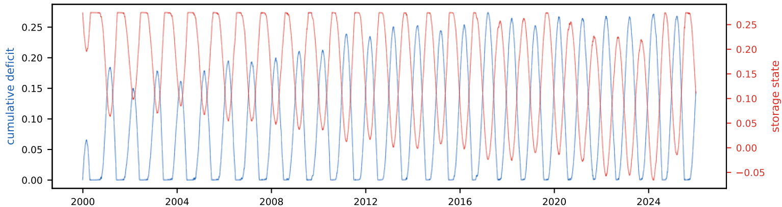
Cumulative deficit & storage state (peak deficit = required storage, S_{\text{tot}} =27.5% of annual)
