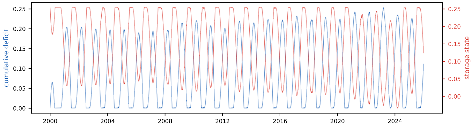
Cumulative deficit & storage state (peak deficit = required storage, S_{\text{tot}} =25.4% of annual)
