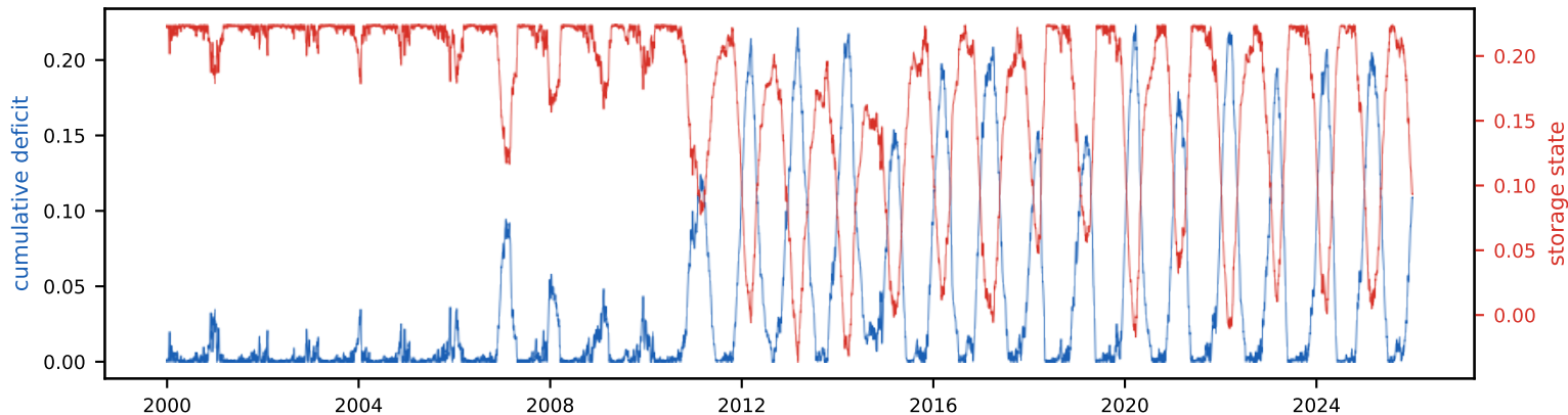
Cumulative deficit & storage state (peak deficit = required storage, S_{\text{tot}} =22.4% of annual)
