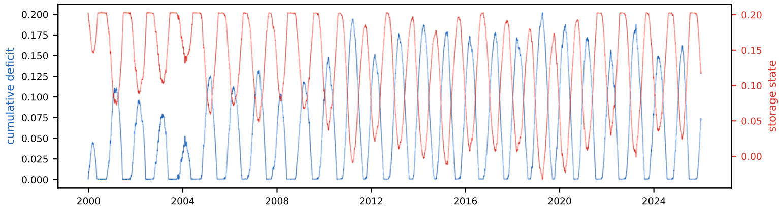
Cumulative deficit & storage state (peak deficit = required storage, S_{\text{tot}} =20.3% of annual)
