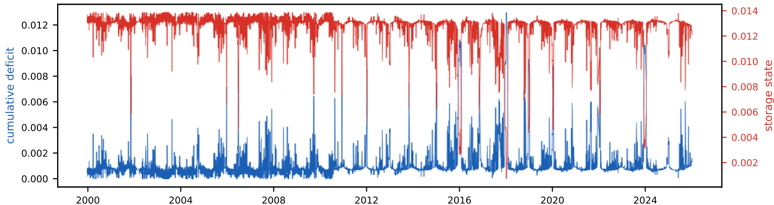
Cumulative deficit & storage state (peak deficit = required storage, S_{\text{tot}} =1.4% of annual)
