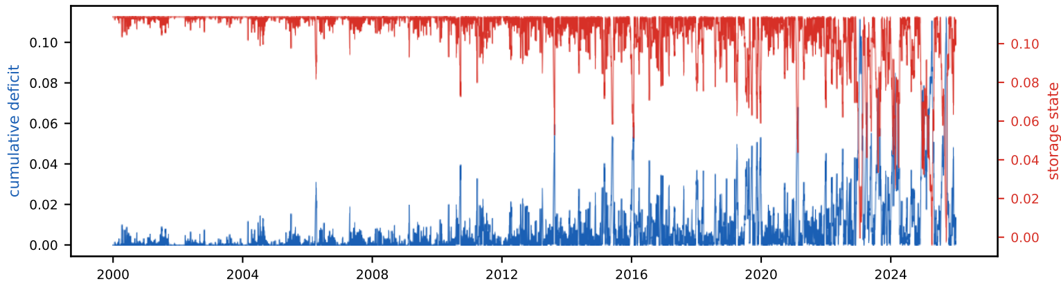
Cumulative deficit & storage state (peak deficit = required storage, S_{\text{tot}} =11.4% of annual)
