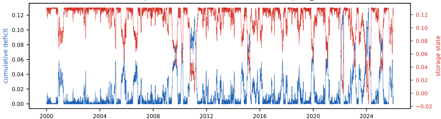
Real energy vs EIA demand (24 TWh/yr, 0.2% land)
